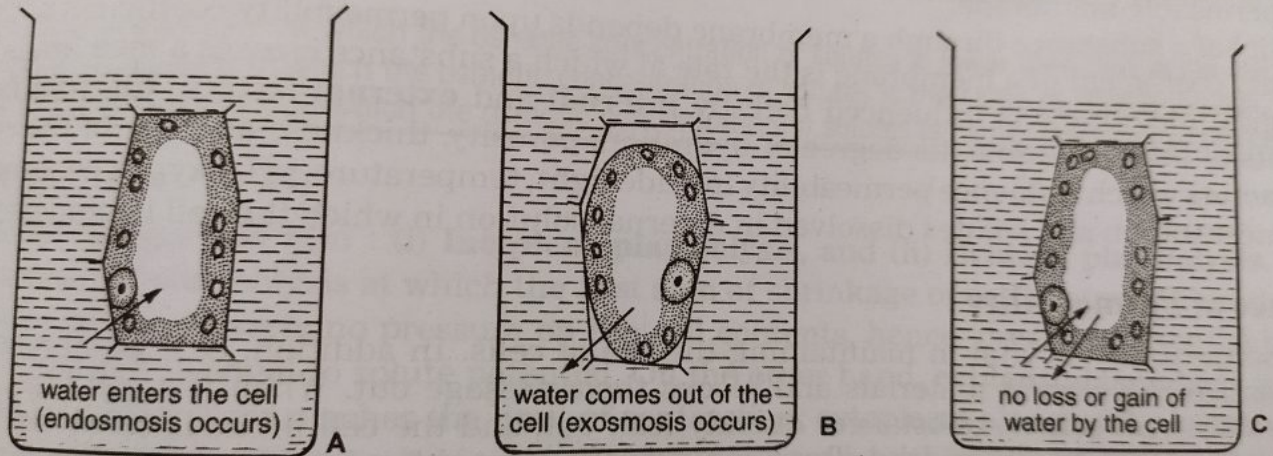
Solutions of different concentrations in relation to cell sap : A. hypotonic solution; B. hypertonic solution; C. isotonic solution
